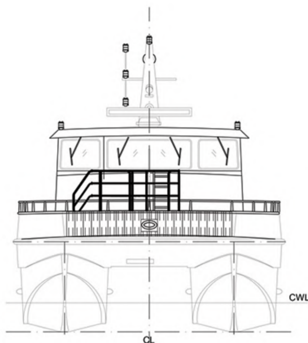
FRONT VIEW
