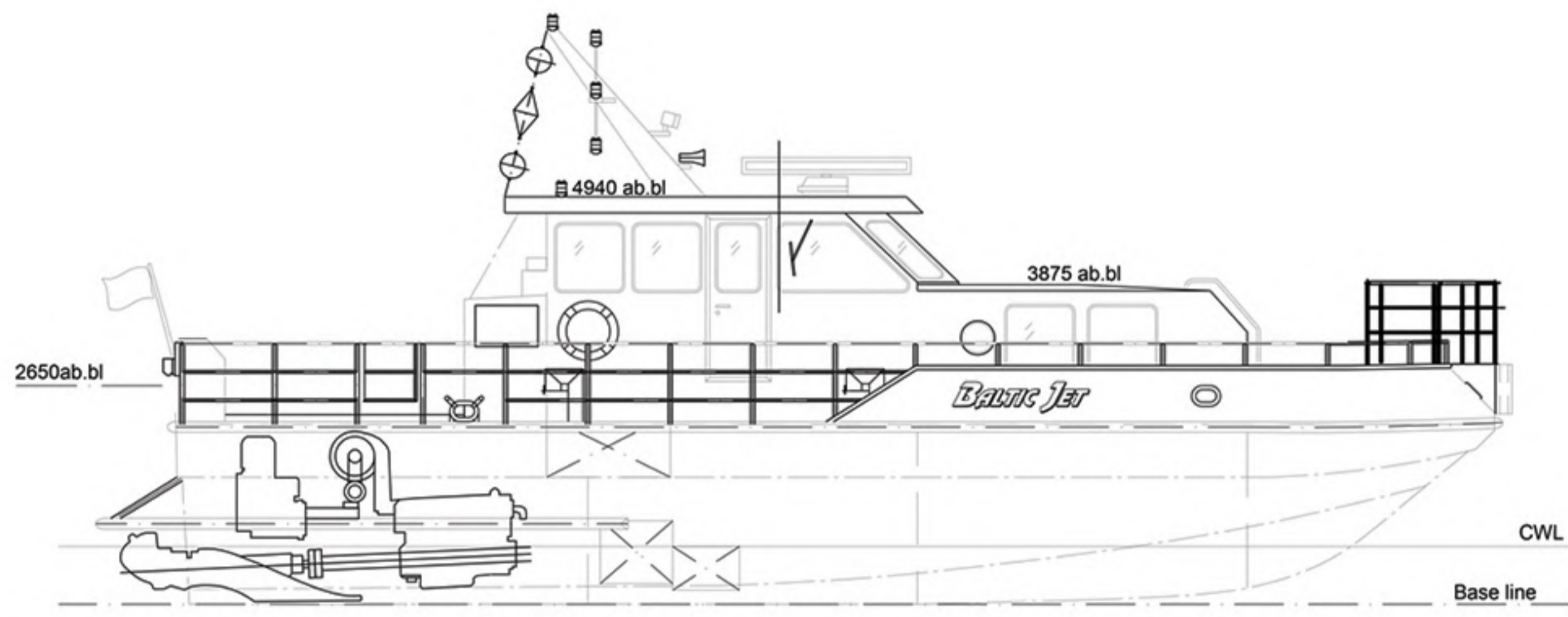
PROFILE
