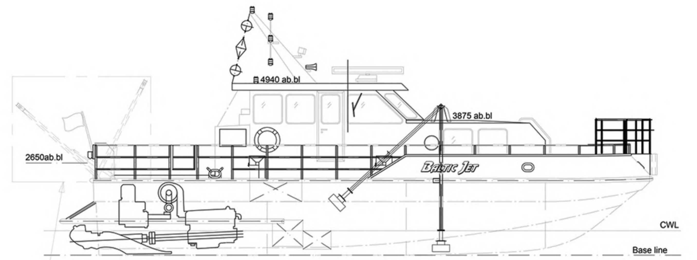
PROFILE
