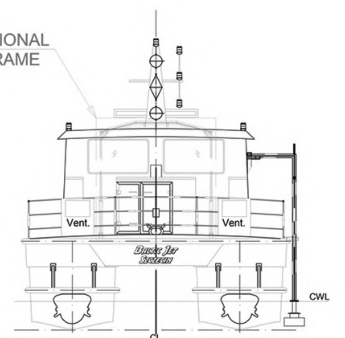
BACK VIEW
